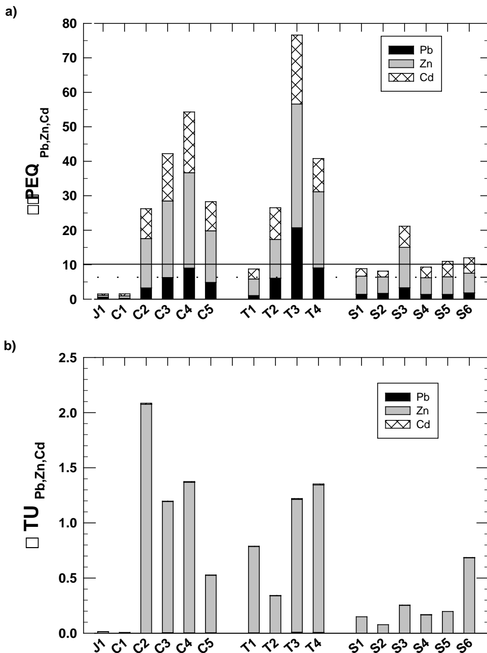
Figure 4. Assessment of risk of metals toxicity in a) <250- \mu m fraction of sediment; and b) surface water. \sum \text{PEQ}_{\text{Pb,Zn,Cd}} = sediment probable-effect concentration quotient ( \sum \text{concentration/probable-effect concentration} ; MacDonald et al. 2000). Lines represent Tri-State Mining District low-risk (dashed) and high-risk (solid) toxicity thresholds (MacDonald et al., 2010). \sum \text{TU}_{\text{Pb,Zn,Cd}} = surface-water toxic unit ( \sum \text{concentration/water-quality criterion} ; USEPA, 2005). Values <1.0 are predicted to be non-toxic.
