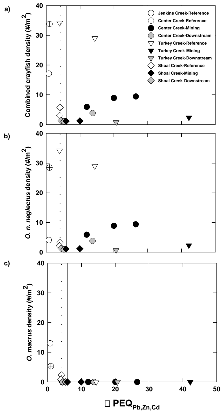
Figure 5. Relationship among sediment probable-effects concentrations quotients ( \sum \text{PEQ}_{\text{Pb,Zn,Cd}} ; MacDonald et al. 2010) and a) combined mean densities of Orconectes neglectus and Orconectes macrus ; b) mean densities of O. n. neglectus ; and c) mean densities of O. macrus . Lines represent Tri-State Mining District low-risk (dashed) and high-risk (solid) toxicity thresholds (MacDonald et al. 2010).
